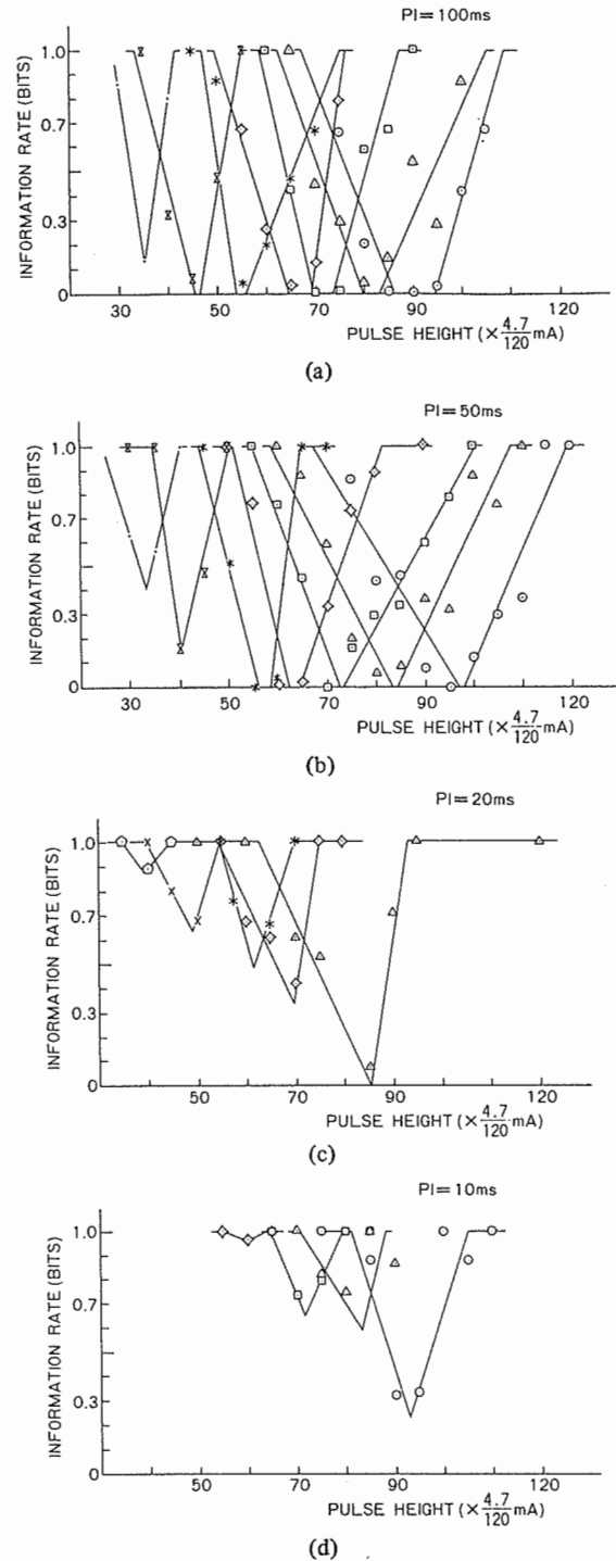
Fig. 3. (a) Detectable difference between stimuli A and B of Fig. 2 for PI = 100 ms. The marks \odot , \triangle , \square , \diamond , \times , \Sigma , and \cdot indicate the results for TB of 150, 200, 250, 300, 400, 800, and 1600 \mu s, respectively. (b) Detectable difference between stimuli A and B of Fig. 2 for PI = 50 ms. (c) Detectable difference between stimuli A and B of Fig. 2 for PI = 20 ms. The symbols \times and \odot indicate the results for TB of 600 and 900 \mu s, respectively. (d) Detectable difference between stimuli A and B of Fig. 2 for PI = 10 ms.
