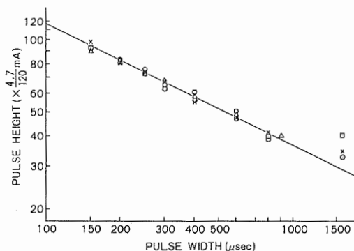
Fig. 4. Plot of the average IB values that indicate the minimum discrimination using a log-log scale as a function of TB . The marks \odot , \times , \triangle , and \square are the results for PI = 100, 50, 20 , and 10 ms, respectively.
